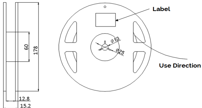
Figure 13: Emitter Reel Drawings
